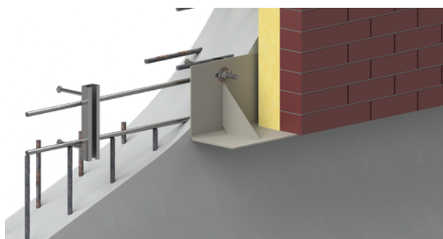
Brickwork connection
