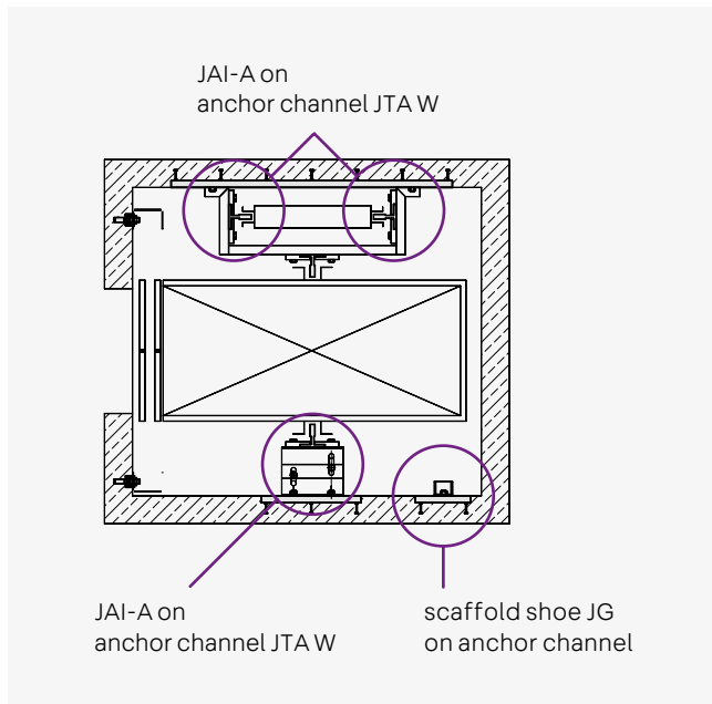
Schematic arrangement of the anchor channels JTA W with elevator insulation JAI
